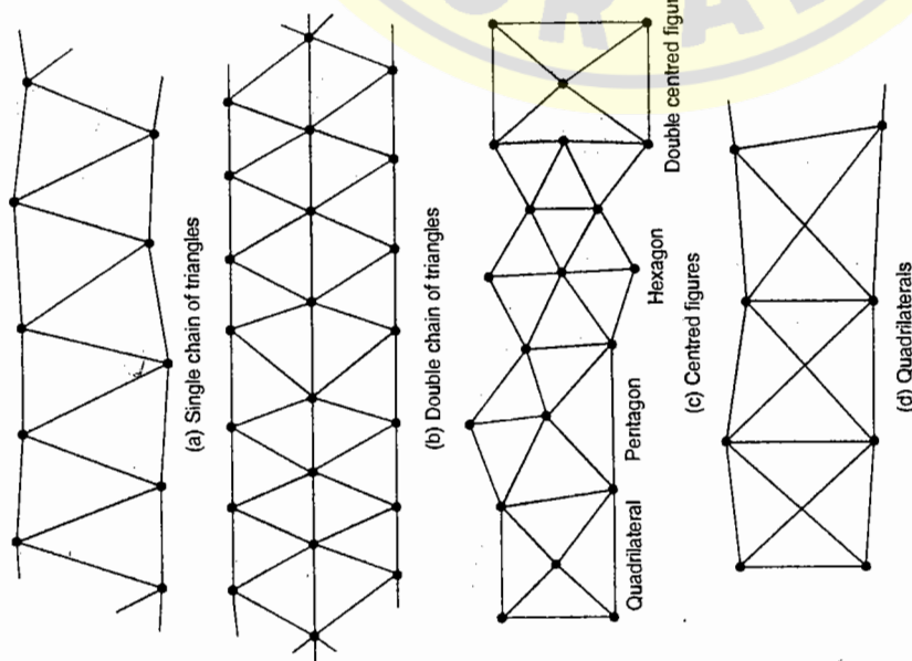
FIG. 8.1. TRIANGULATION FIGURES.
