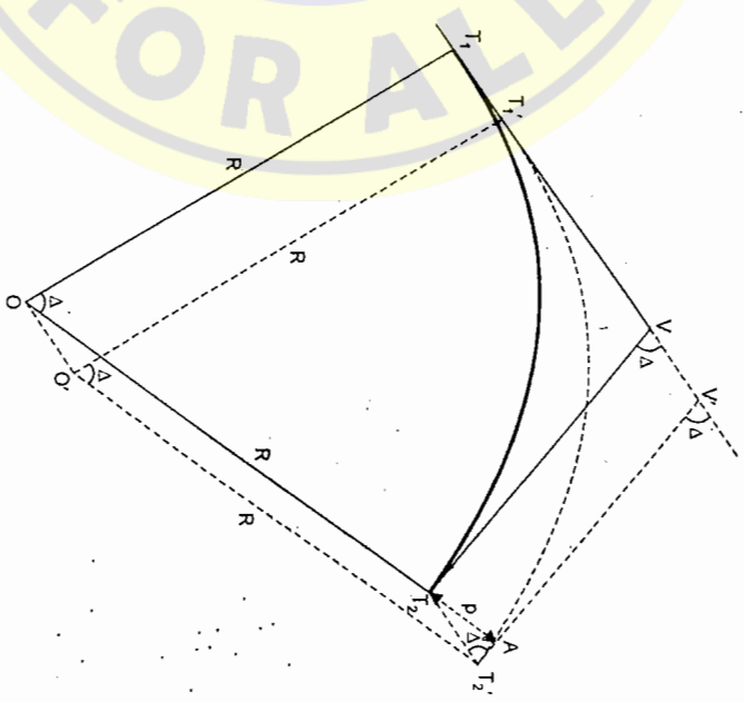
FIG. 1.21. SHIFTING FORWARD TANGENT OUTWARD (SAME RADIUS)
