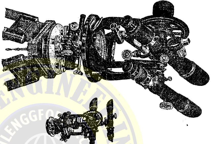
FIG. 7.1. MINING TRANSIT SHOWING THE AUXILIARY TELESCOPE IN BOTH POSITIONS.
