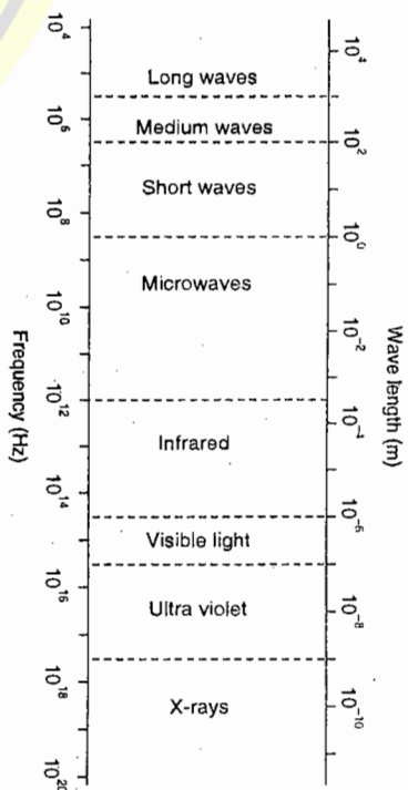
FIG. 15.2 ELECTROMAGNETIC SPECTRUM.
