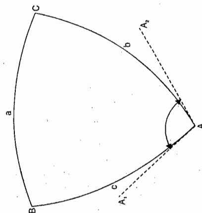
FIG. 13.13. SPHERICAL TRIANGLE.
