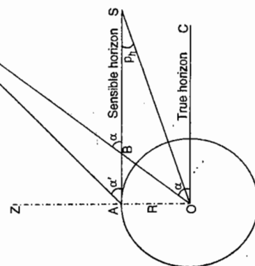
FIG. 13.35 SUN'S PARALLAX.
