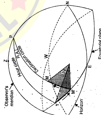
FIG. 13.7. THE DECLINATION-RIGHT ASCENSION SYSTEM.
